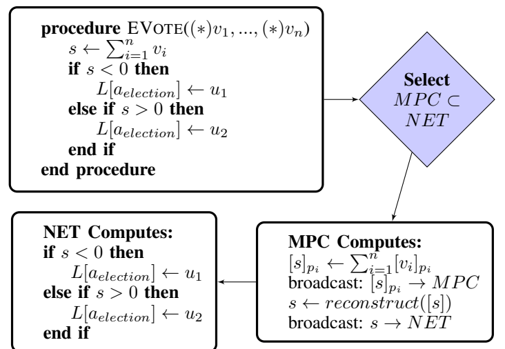
Fig. 2. Example of a flow of secure computation in a blockchain network. The top left block (EVote procedure) is the insecure code, where the arguments marked in (*) are private and stored as shares on the DHT. The network selects a subset of nodes at random to compute a secure version of EVote and broadcasts the results back to the entire network, that stores it on the ledger.
